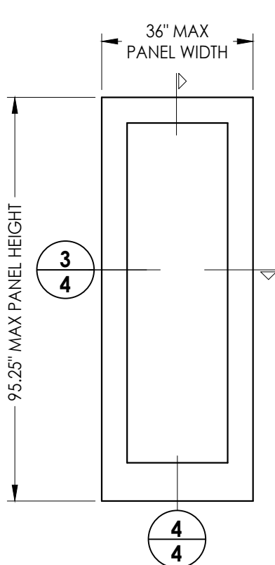
FIBERGLASS DOOR/SIDELITE PANEL Therma-Tru 8'-0" (Wood Edge)
