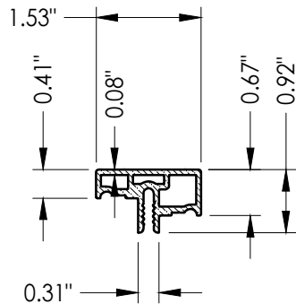
2B EXTERIOR FRAME 1-1/4" GLAZING
