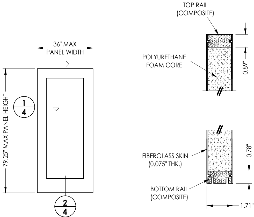
FIBERGLASS DOOR/SIDELITE PANEL Therma-Tru 6'-8" (Wood Edge)
